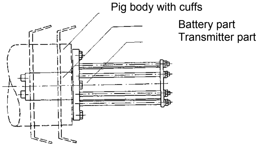
Fig. 1: Installation of the pig transmitter (schematic representation). The transmitter part remains free.
